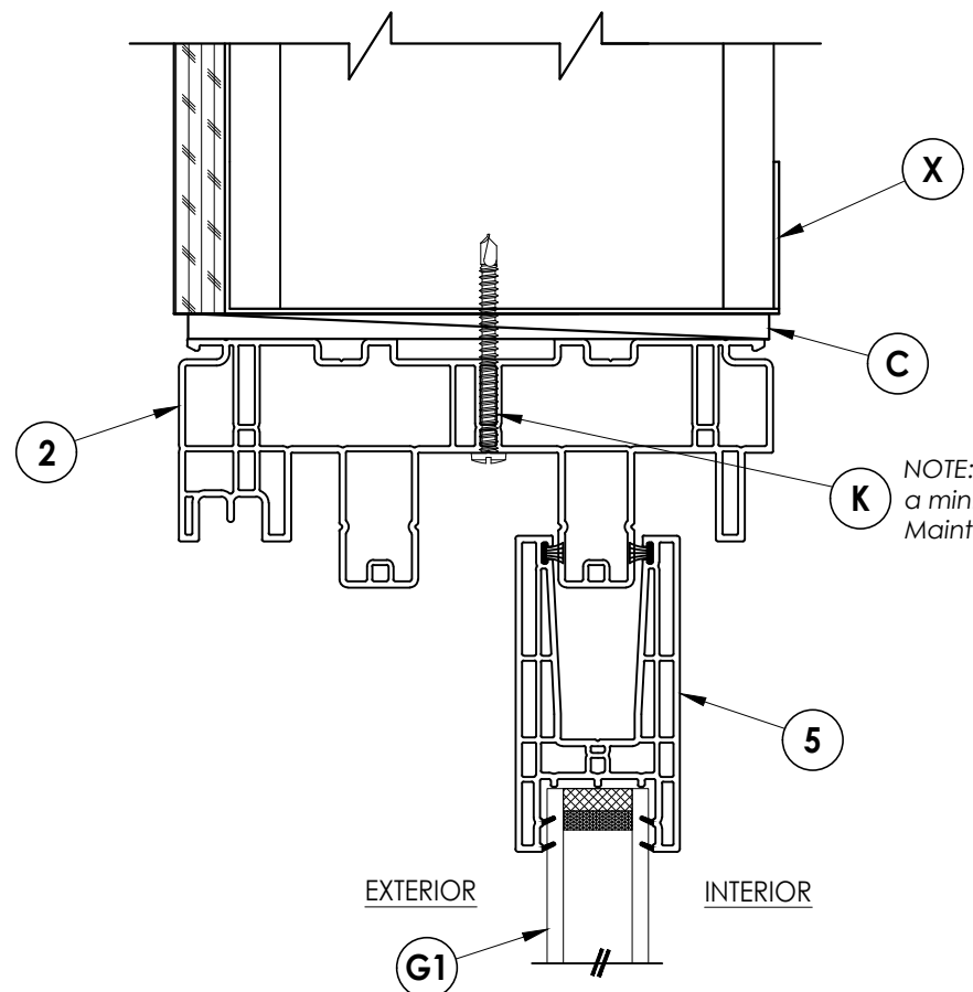
2 VERTICAL CROSS SECTION 3 Shown w/ Steel Stud Framing
