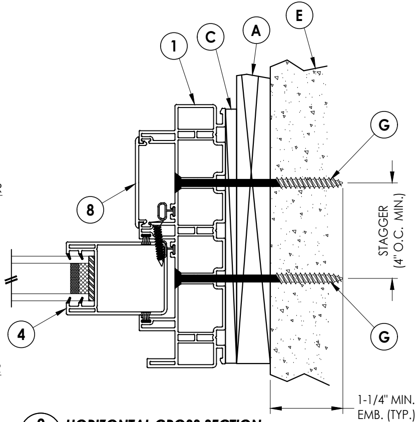
2 HORIZONTAL CROSS SECTION 2 Shown w/ 1X Buck Construction
