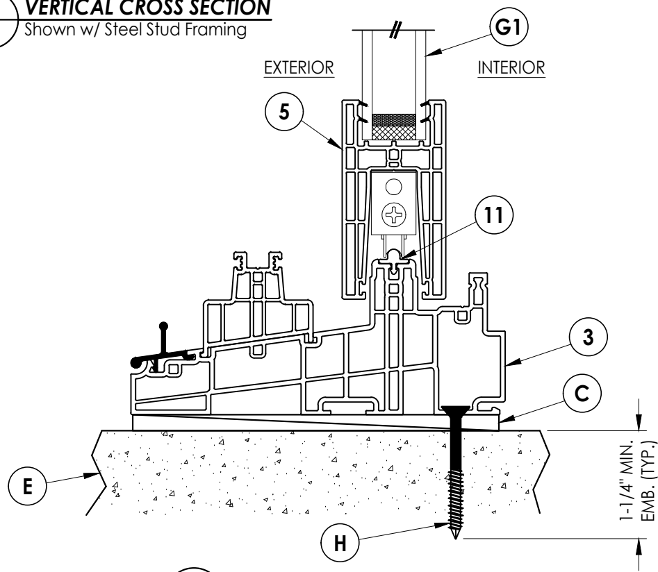
3 VERTICAL CROSS SECTION 3 Shown Direct to Masonry
